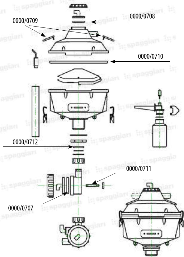
TECHNICAL DRAWING (FOR REFERENCE PURPOSE ONLY)
